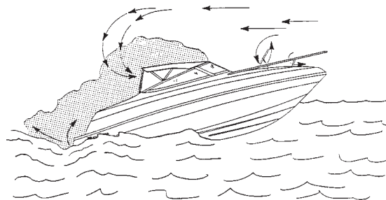
Figure B10: Inefficient trim angles.
