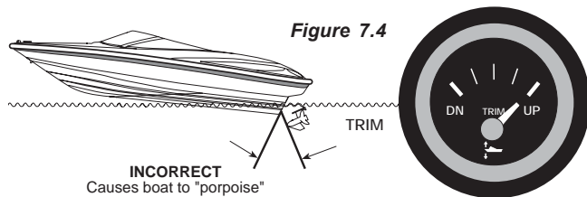
Figures 7.2-7.4: Trimming the Boat with Outdrive
