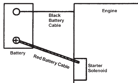
Figure H1: Single Engine-Single Battery Installation
