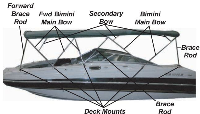
Figure O2: 234/264 FS Forward Bimini & Bimini Top
