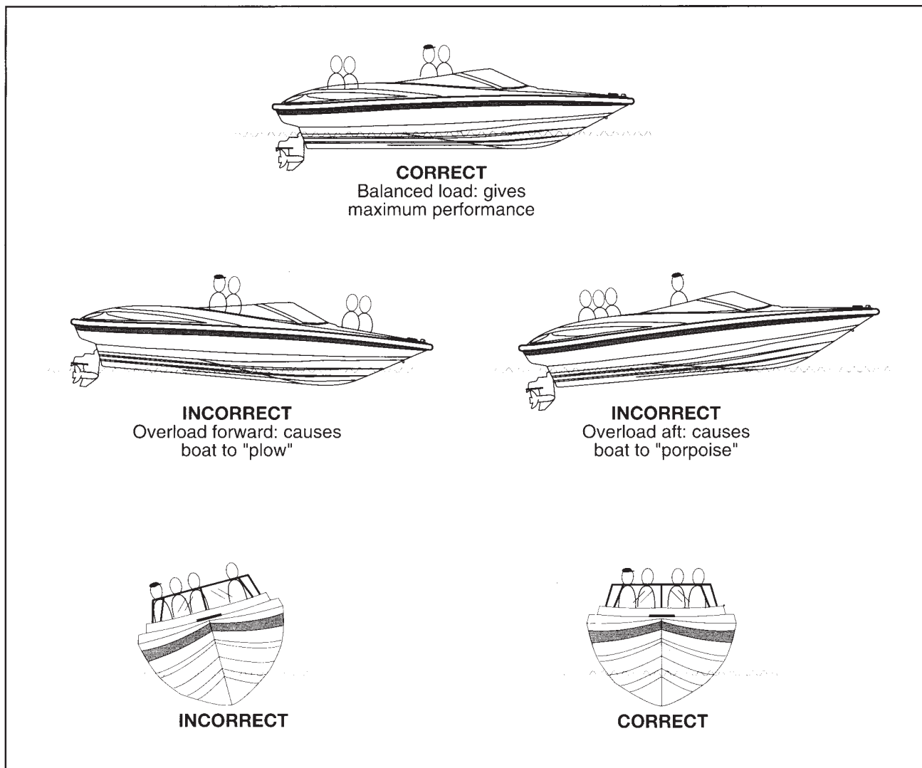
Figure 7.1: Loading Passengers and Gear
