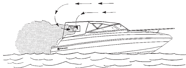
Figure B9: Backdrafting - Air flows over boat and behind transom.
