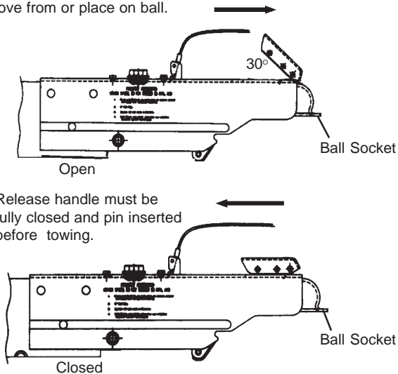
Figure S6: Surge Brake Actuator & Coupling Assembly
