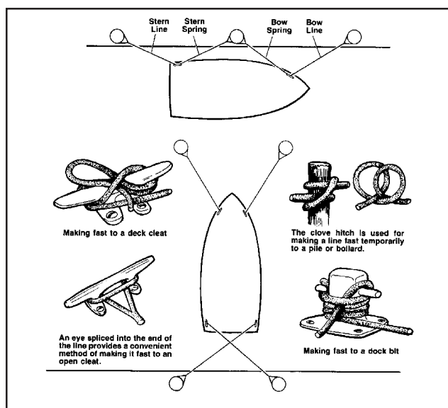
Figure 7.5: Mooring Lines
