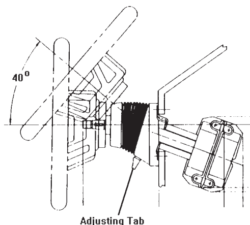
Figure G1: Tilt Steering Option
