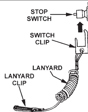
Figure E20: Emergency Stop Switch
