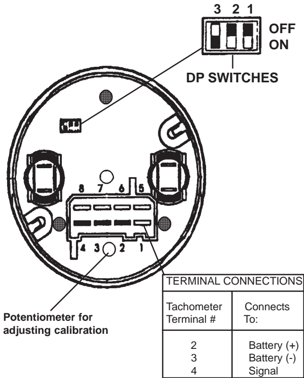
Figure E5: 214 Candia FS I/O Tachometer-Rear View
