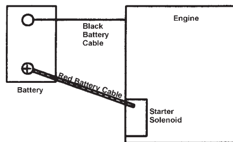
Figure H1: Single Engine-Single Battery Installation
