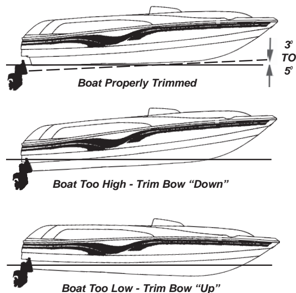
Figure E2: Running Angle
