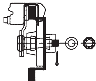
Figure S5: Brake Actuator & Coupling Assembly and Disc Brake
