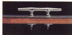
Wood backing at all through-the-hull-and-deck fastening points and through-bolting of stainless steel cleats and rails to metal backing plates provides greater durability and strength.
