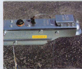
Trailer coupler with safety chains and brake actuator
