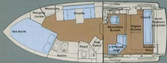
Mid-Ship Dinette/Cockpit Seating
