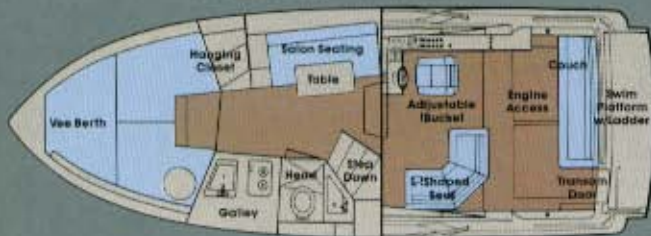
Cockpit Seating/Mid-Ship Salon
